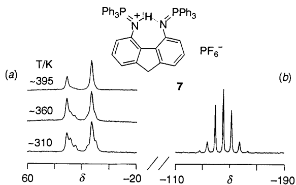
Fig. 1 Variable temperature ^{31}\text{P} MAS NMR spectra of compound 7 , 4 \mu\text{s} ^{31}\text{P} 90^\circ pulses, 50 kHz sweep width, 5 s recycle delay, ^1\text{H} decoupling during acquisition. (a) Signals of the iminophosphorane fragments at different temperatures. (b) Signal of the counterion \text{PF}_6^-
